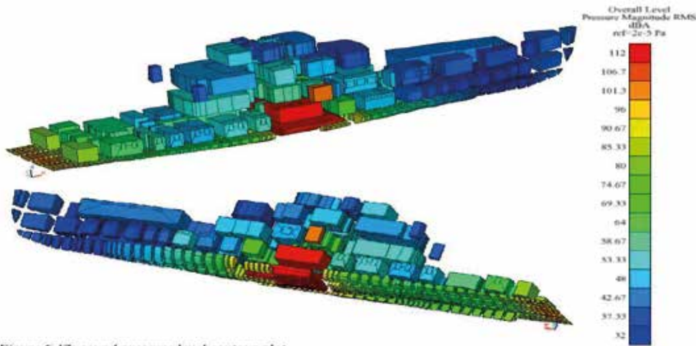
Figure 6.17: sound pressure level contour plot
